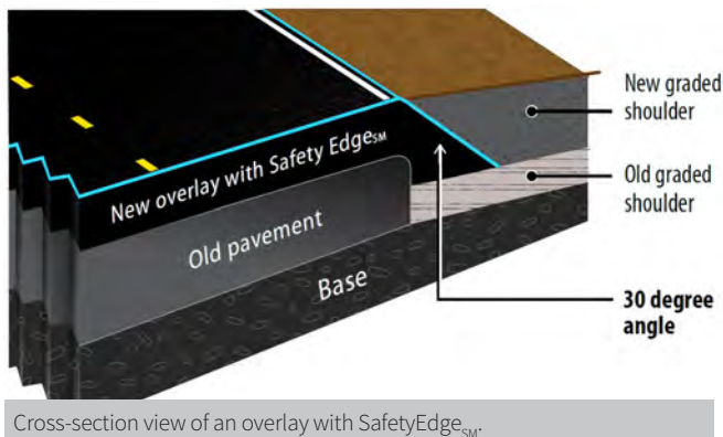
Cross-section view of an overlay with SafetyEdge SM .
